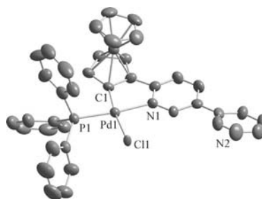
Figure 8. Molecular structure of 17 (one of the two independent molecules). Thermal ellipsoids are drawn at 50% probability. H atoms and CH 2 Cl 2 are omitted for clarity. Selected bond lengths [Å] and angles [°] (corresponding values for the second independent molecule are given in brackets): Pd(1)-C(1) 1.990(7) [1.992(7)], Pd(1)-N(1) 2.150(5) [2.141(5)], Pd(1)-P(1) 2.2454(18) [2.2398(17)], Pd(1)-Cl(1) 2.4713(13) [2.4213(14)] and C(1)-Pd(1)-N(1) 80.9(2) [80.9(3)], C(2)-Pd(1)-P(1) 92.3(2) [92.0(2)], P(1)-Pd(1)-Cl(1) 93.80(6) [94.58(6)], N(1)-Pd(1)-Cl(1) 93.06(15) [93.64(15)].
