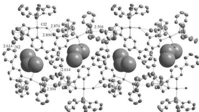
Figure 9. 2D lamellar structure of 17 showing the C–H \cdots Cl(N) interactions. Thermal ellipsoids are drawn at 50% probability. Non-hydrogen bonding H atoms are omitted for clarity.
