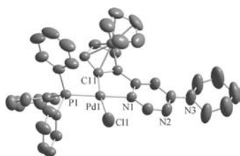
Figure 11. Molecular structure of 27 . Thermal ellipsoids are drawn at 50% probability. Non-hydrogen bonding H atoms are omitted for clarity. Selected bond lengths [Å] and angles [°]: Pd(1)–C(11) 1.987(8), Pd(1)–N(1) 2.114(3), Pd(1)–P(1) 2.2345(9), Pd(1)–Cl(1) 2.3685(2) and C(11)–Pd(1)–N(1) 80.78(12), C(11)–Pd(1)–P(1) 93.18(10), P(1)–Pd(1)–Cl(1) 94.80(4), N(1)–Pd(1)–Cl(1) 91.95(7).
