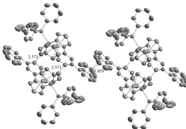
Figure 3. 1D chain structure of 3 ·2CH 2 Cl 2 showing the C–H···N hydrogen bonds and \pi – \pi interactions. Thermal ellipsoids are drawn at 50% probability. Non-hydrogen bonding H atoms and CH 2 Cl 2 are omitted for clarity.
