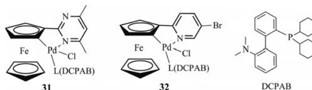
Figure 1. Ferrocenyl palladacycles 31 and 32 .
