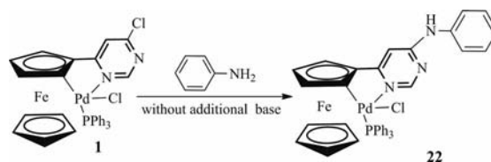
Scheme 5. Synthesis of 22 .
