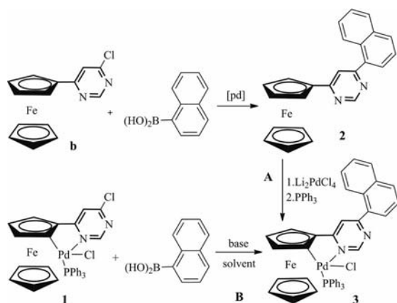
Scheme 2. Synthesis of 3 .
