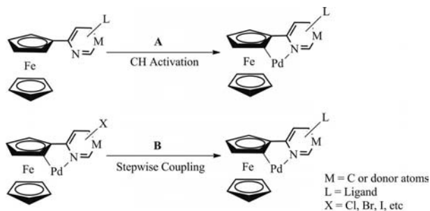
Scheme 1. Synthetic strategy for palladacycles with polydentate ligands.
