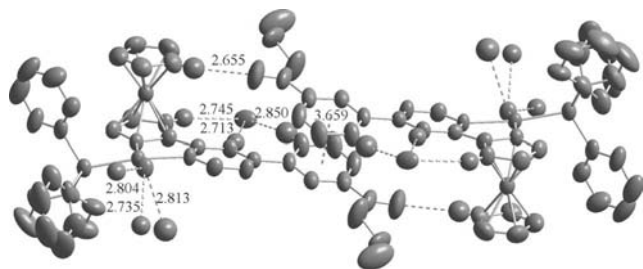
Figure 6. Two-dimensional lamellar structure of 11 showing the C-H \cdots Cl(O) hydrogen bonds and \pi - \pi interactions. Thermal ellipsoids are drawn at 50% probability. Non-hydrogen bonding H atoms are omitted for clarity.
