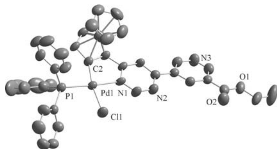
Figure 5. Molecular structure of 11 (one of the two independent molecules). Thermal ellipsoids are drawn at 50% probability. H atoms are omitted for clarity. Selected bond lengths [Å] and angles [°] (corresponding values for the second independent molecule are given in brackets): Pd(1)-C(2) 1.983(4) [1.981(4)], Pd(1)-N(1) 2.127(3) [2.131(3)], Pd(1)-P(1) 2.2442(13) [2.2235(13)], Pd(1)-Cl(1) 2.3740(12) [2.3856(12)] and C(2)-Pd(1)-N(1) 80.70 (15) [81.02(15)], C(2)-Pd(1)-P(1) 92.28(13) [90.57(13)], P(1)-Pd(1)-Cl(1) 97.01(5) [95.67(4)], N(1)-Pd(1)-Cl(1) 90.28(10) [94.54(10)].
