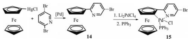
Scheme 4. Synthesis of 14 and 15 .
