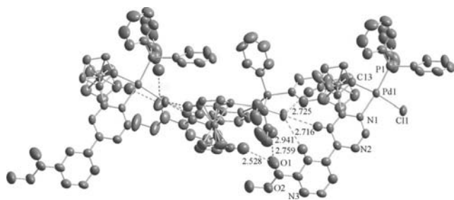
Figure 4. 1D chain structure of 10 showing the C-H \cdots Cl(O) hydrogen bonds. Thermal ellipsoids are drawn at 50% probability. Non-hydrogen bonding H atoms are omitted for clarity. Selected bond lengths [Å] and angles [°]: Pd(1)-C(13) 1.994(7), Pd(1)-N(1) 2.127(6), Pd(1)-P(1) 2.242(2), Pd(1)-Cl(1) 2.379(2) and C(13)-Pd(1)-N(1) 80.8(3), C(13)-Pd(1)-P(1) 92.3(2), P(1)-Pd(1)-Cl(1) 95.90(8), N(1)-Pd(1)-Cl(1) 91.79(17).
