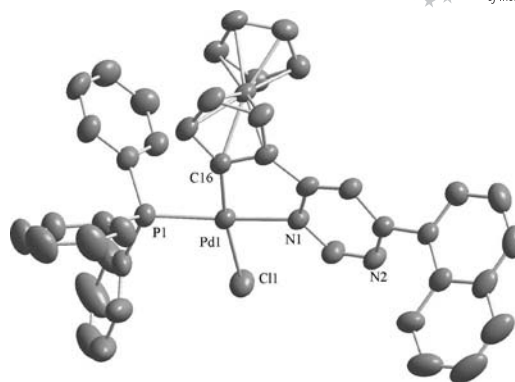
Figure 2. Molecular structure of 3 ·2CH 2 Cl 2 . Thermal ellipsoids are drawn at 50% probability. H atoms and CH 2 Cl 2 are omitted for clarity. Selected bond lengths [Å] and angles [°]: Pd(1)–C(16) 1.999(5), Pd(1)–N(1) 2.130(4), Pd(1)–P(1) 2.2402(14), Pd(1)–Cl(1) 2.3842(15) and C(16)–Pd(1)–N(1) 80.80(18), C(16)–Pd(1)–P(1) 92.11(15), P(1)–Pd(1)–Cl(1) 95.30(5), N(1)–Pd(1)–Cl(1) 91.93(12).
