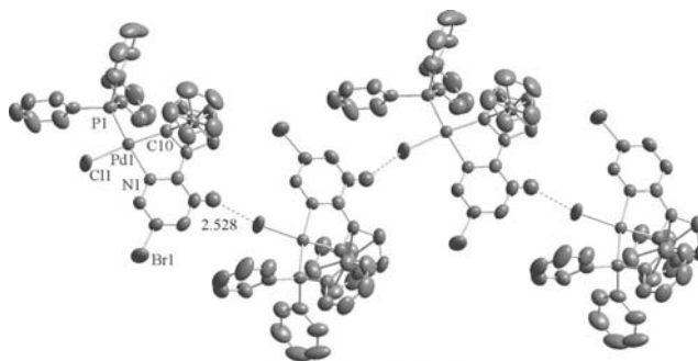
Figure 7. 1D chain structure of 15 showing the C-H \cdots Cl hydrogen bonds. Thermal ellipsoids are drawn at 50% probability. Non-hydrogen bonding H atoms are omitted for clarity. Selected bond lengths [Å] and angles [°]: Pd(1)-C(10) 1.988(4), Pd(1)-N(1) 2.140(3), Pd(1)-P(1) 2.2322(11), Pd(1)-Cl(1) 2.3642(2) and C(10)-Pd(1)-N(1) 81.38(15), C(10)-Pd(1)-P(1) 90.34(12), P(1)-Pd(1)-Cl(1) 94.81(4), N(1)-Pd(1)-Cl(1) 91.80(9).
