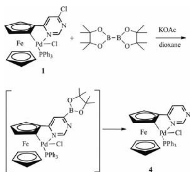
Scheme 3. Reaction of bis(pinacolato)diboron and 1 .
