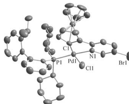
Figure 13. Molecular structure of 32 . Thermal ellipsoids are drawn at 50% probability. H atoms and CH 2 Cl 2 are omitted for clarity. Selected bond lengths [Å] and angles [°]: Pd(1)–C(1) 1.973(6), Pd(1)–N(1) 2.156(5), Pd(1)–P(1) 2.2679(15), Pd(1)–Cl(1) 2.3986(15) and C(1)–Pd(1)–N(1) 79.9(2), C(1)–Pd(1)–P(1) 95.25(17), P(1)–Pd(1)–Cl(1) 93.28(6), N(1)–Pd(1)–Cl(1) 92.21(13).
