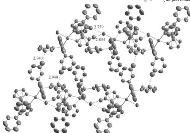
Figure 12. 2D lamellar structure of 27 showing the C–H \cdots Cl( \pi ) interactions. Thermal ellipsoids are drawn at 50% probability. Non-hydrogen bonding H atoms are omitted for clarity.
