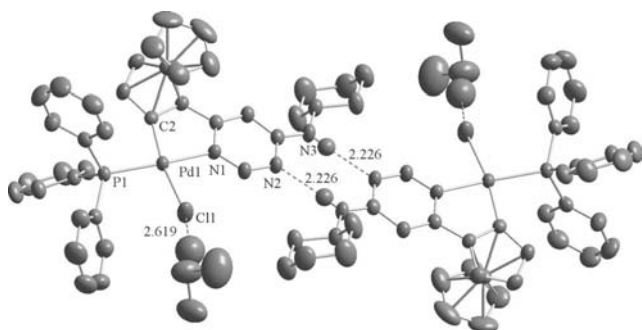
Figure 10. The dimeric structure of 26 showing the C–H \cdots N hydrogen bonds. Thermal ellipsoids are drawn at 50% probability. Non-hydrogen bonding H atoms are omitted for clarity. Selected bond lengths [Å] and angles [°]: Pd(1)–C(2) 1.991(3), Pd(1)–N(1) 2.118(2), Pd(1)–P(1) 2.2407(8), Pd(1)–Cl(1) 2.3818(9) and C(2)–Pd(1)–N(1) 80.63(11), C(2)–Pd(1)–P(1) 92.75(9), P(1)–Pd(1)–Cl(1) 95.56(3), N(1)–Pd(1)–Cl(1) 91.85(7).
