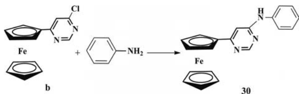
Scheme 6. Synthesis of 30 .
